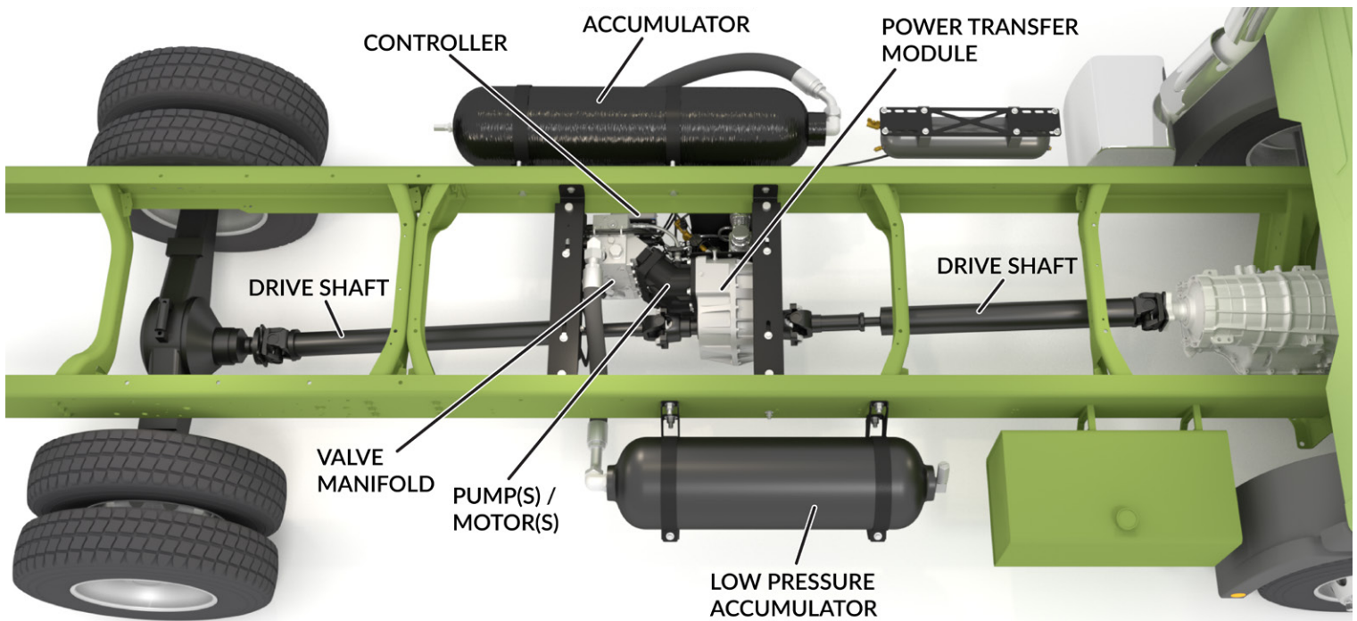
The Lightning Hybrids ERS (Energy Recovery System)
